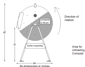
The Actium Batch Compost Drum
